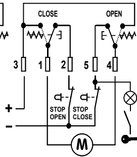
MOTOR DIRECT WITH STOP SWITCH
