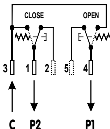
DOUBLE BUTTON
