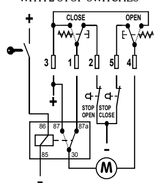
AUTOMATIC STEP RETRACT WITH 2 STOP SWITCHES
