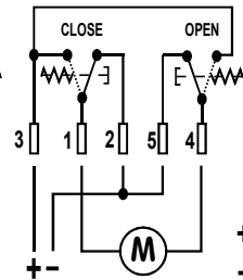
MOTOR DIRECT
