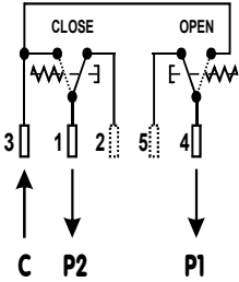
DOUBLE BUTTON
