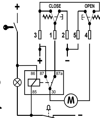
AUTOMATIC STEP RETRACT
