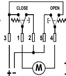
MOTOR DIRECT
