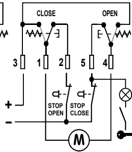
MOTOR DIRECT WITH STOP SWITCH
